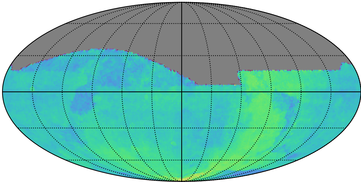
extra_ss_neo4_v3.4_10yrs All sky: Parallax Coverage @ 24.0
