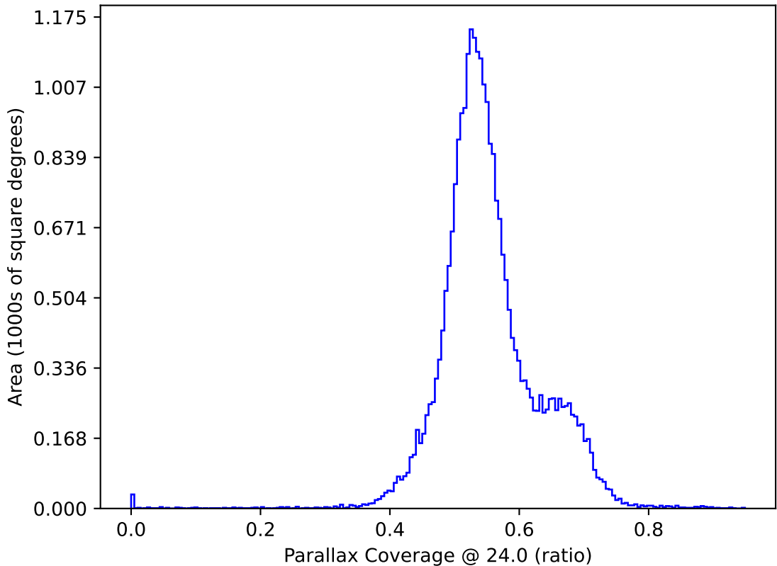
extra_ss_neo4_v3.4_10yrs All sky: Parallax Coverage @ 24.0
