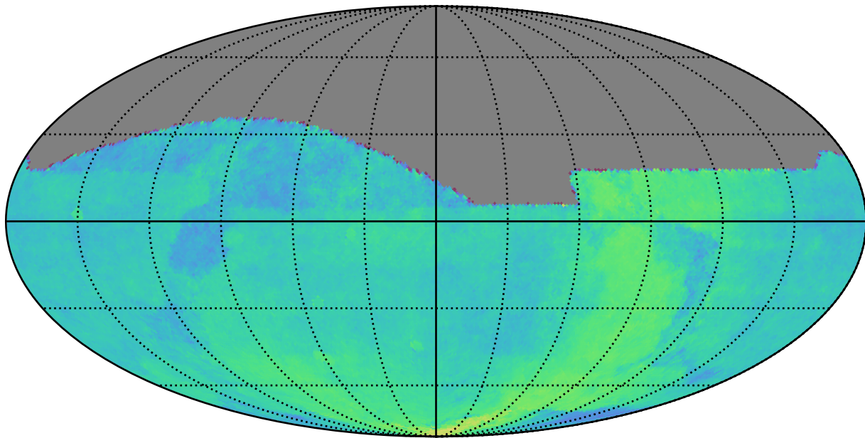
extra_ss_neo4_v3.4_10yrs All sky: Parallax Coverage @ 22.4
