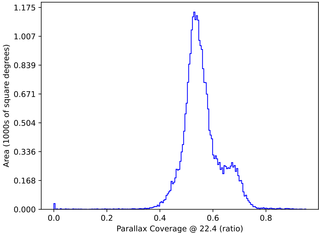
extra_ss_neo4_v3.4_10yrs All sky: Parallax Coverage @ 22.4
