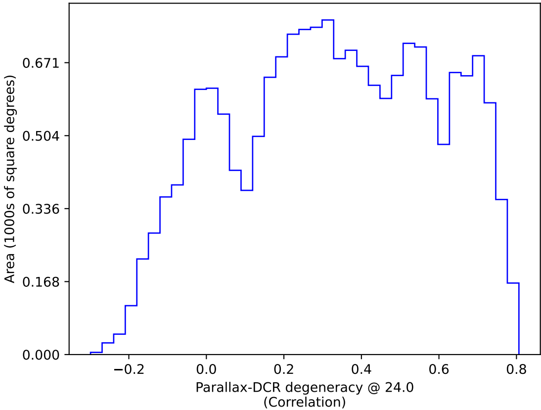
extra_ss_neo4_v3.4_10yrs WFD: Parallax-DCR degeneracy @ 24.0
