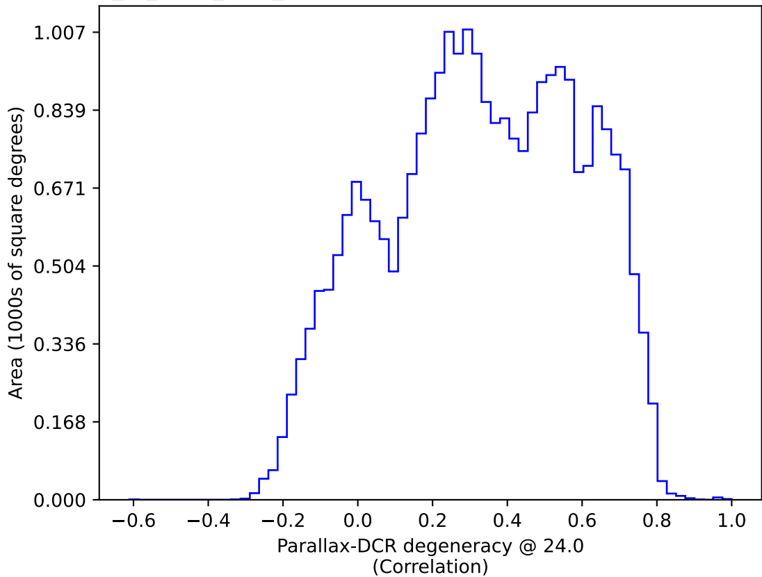
extra_ss_neo4_v3.4_10yrs All sky: Parallax-DCR degeneracy @ 24.0
