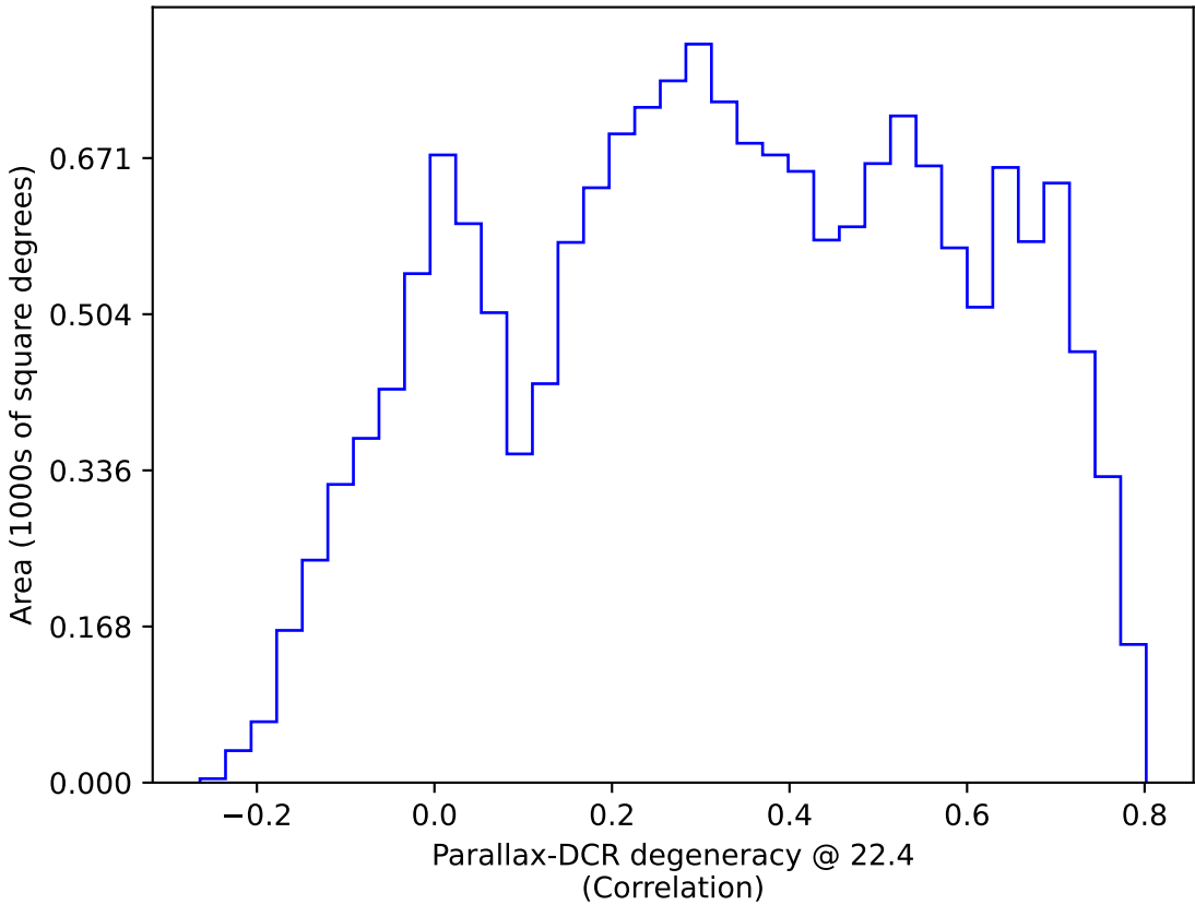
extra_ss_neo4_v3.4_10yrs WFD: Parallax-DCR degeneracy @ 22.4
