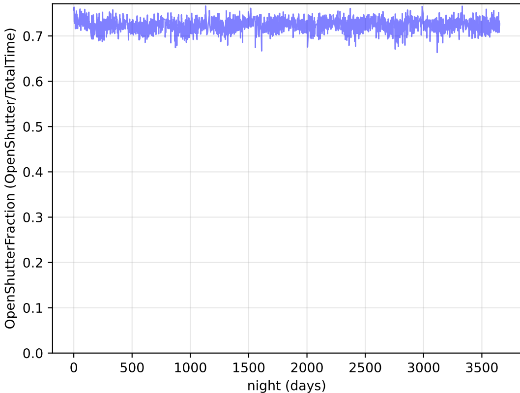
extra_ss_neo4_v3.4_10yrs Per night: OpenShutterFraction
