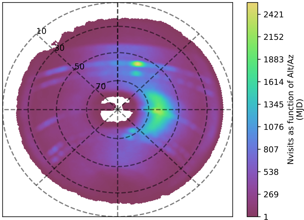
extra_ss_neo4_v3.4_10yrs z band: Nvisits as function of Alt/Az
