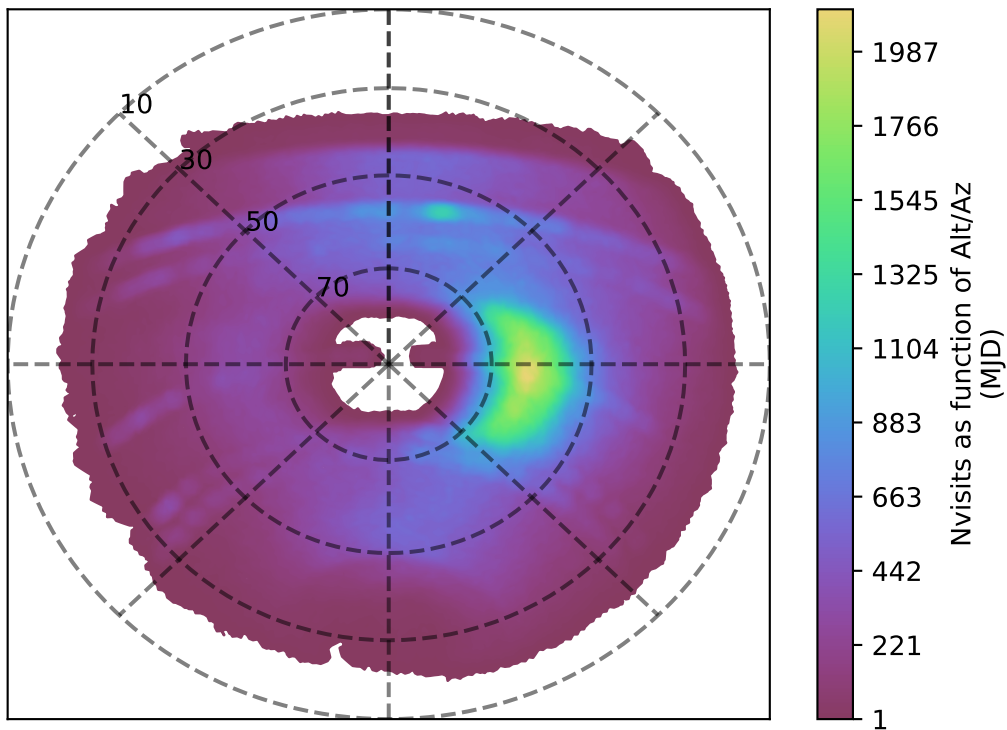
extra_ss_neo4_v3.4_10yrs y band: Nvisits as function of Alt/Az
