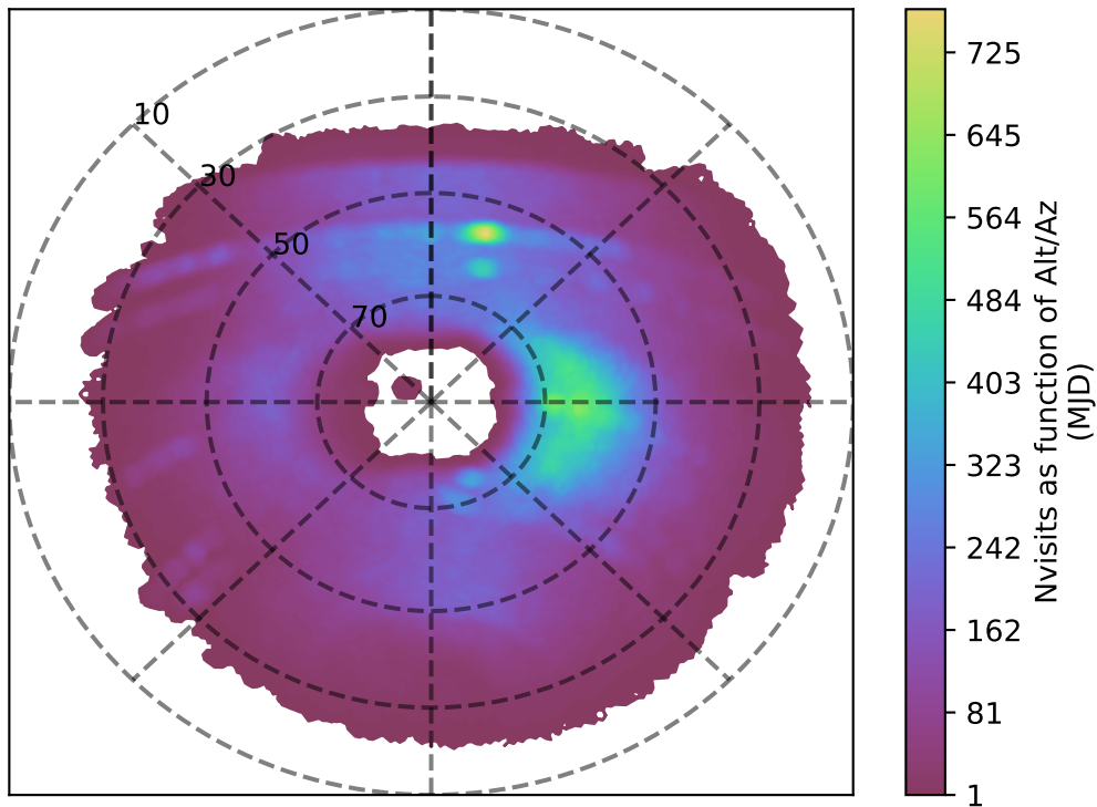
extra_ss_neo4_v3.4_10yrs u band: Nvisits as function of Alt/Az
