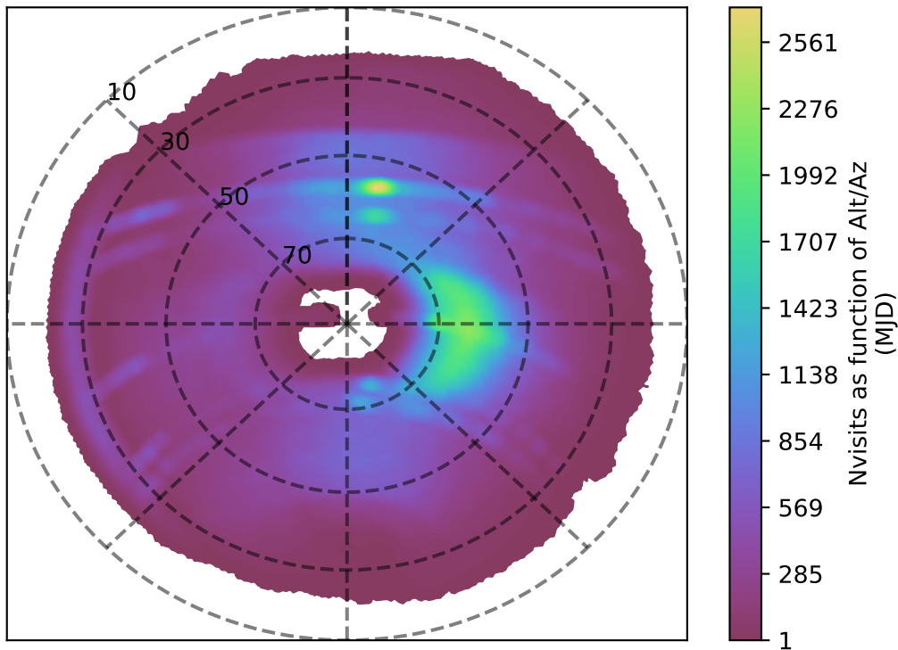
extra_ss_neo4_v3.4_10yrs r band: Nvisits as function of Alt/Az
