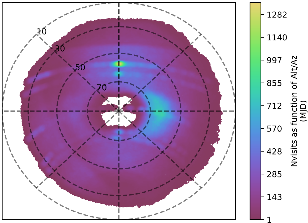
extra_ss_neo4_v3.4_10yrs g band: Nvisits as function of Alt/Az
