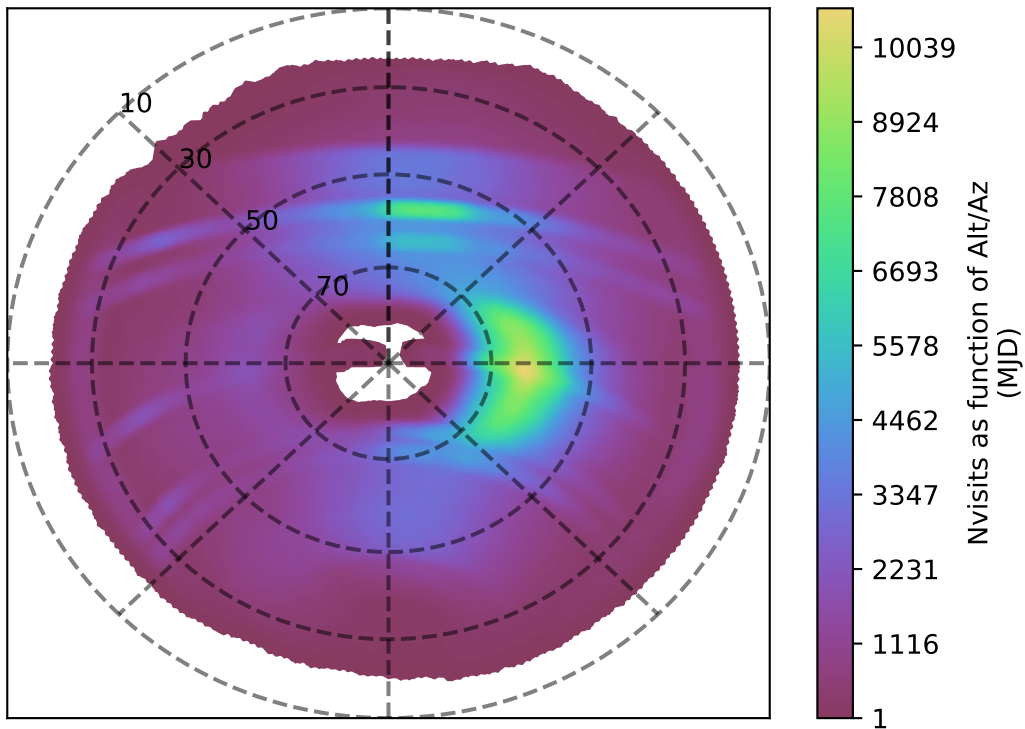
extra_ss_neo4_v3.4_10yrs all bands: Nvisits as function of Alt/Az
