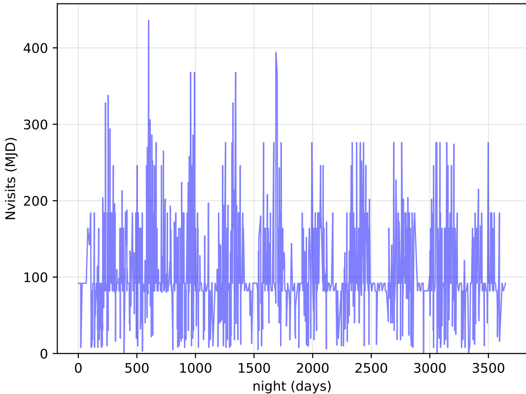
extra_ss_neo4_v3.4_10yrs DDF: Nvisits
