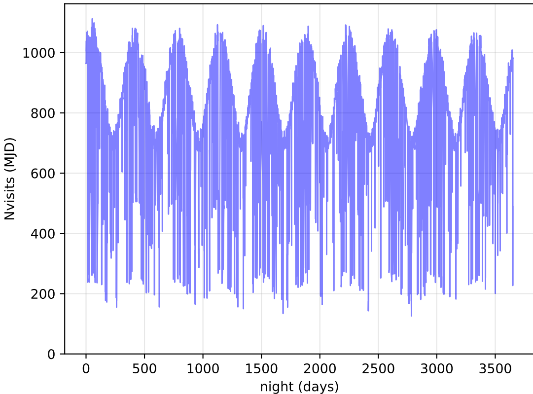
extra_ss_neo4_v3.4_10yrs All visits: Nvisits
