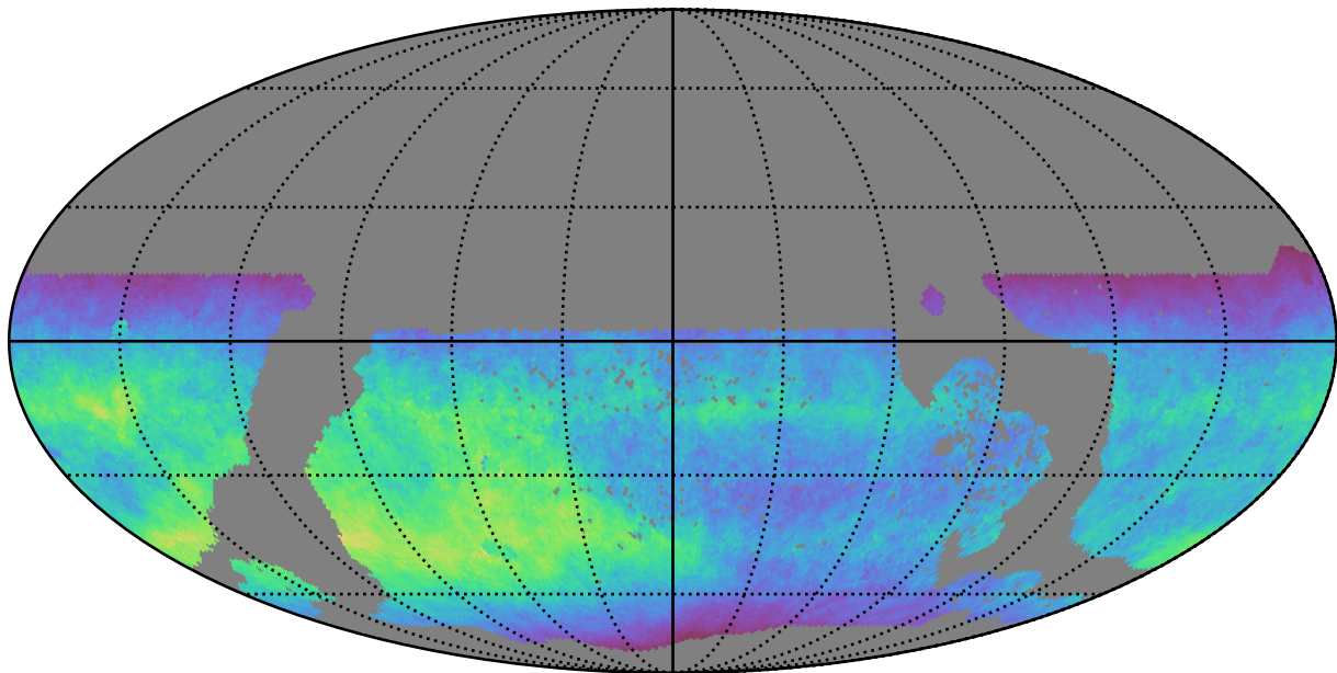
extra_ss_neo4_v3.4_10yrs WFD z band: Normalized Teff
