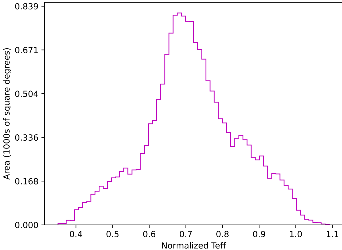
extra_ss_neo4_v3.4_10yrs WFD z band: Normalized Teff
