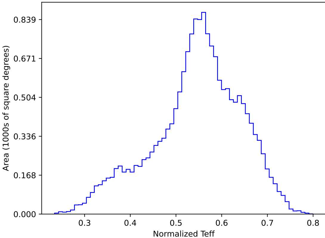
extra_ss_neo4_v3.4_10yrs WFD y band: Normalized Teff
