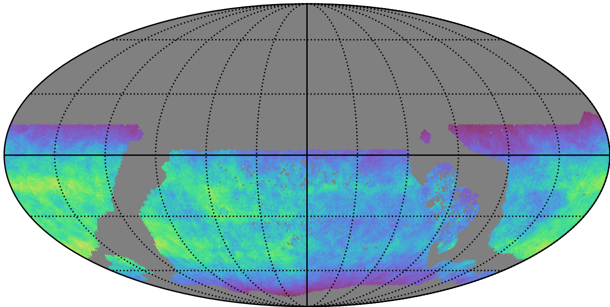
extra_ss_neo4_v3.4_10yrs WFD u band: Normalized Teff
