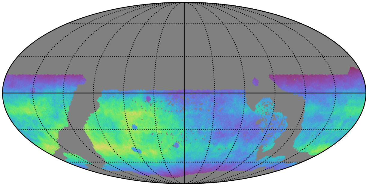
extra_ss_neo4_v3.4_10yrs WFD r band: Normalized Teff
