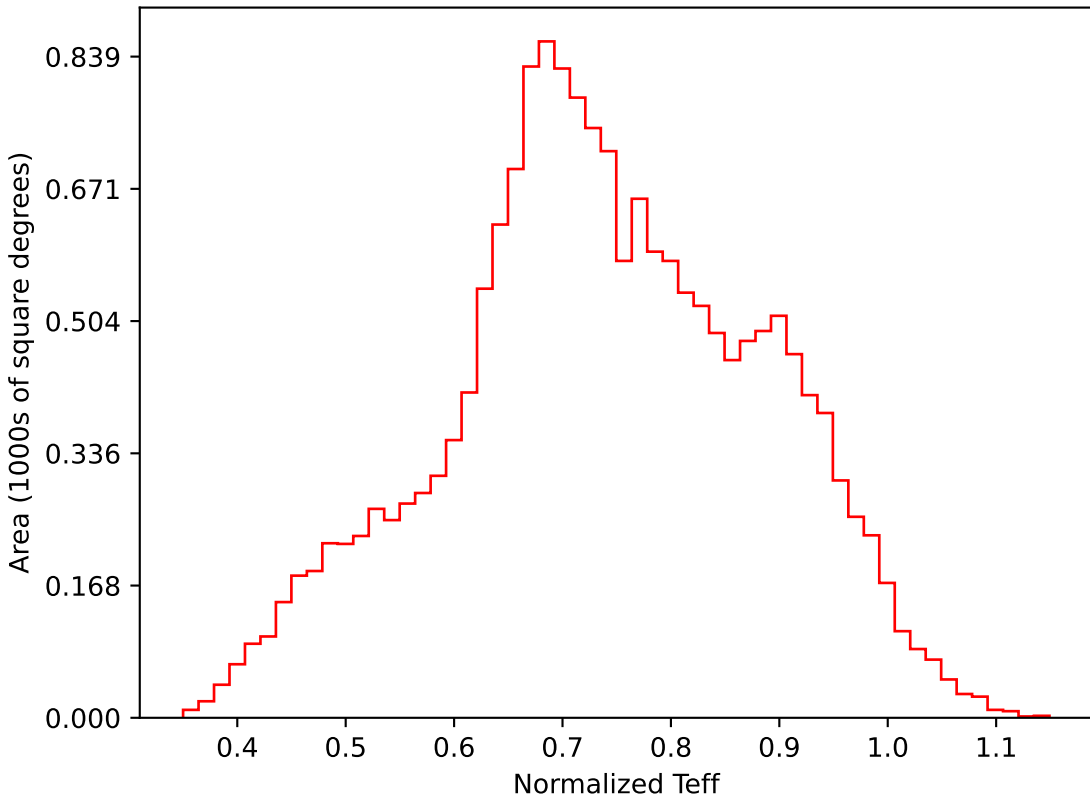
extra_ss_neo4_v3.4_10yrs WFD i band: Normalized Teff
