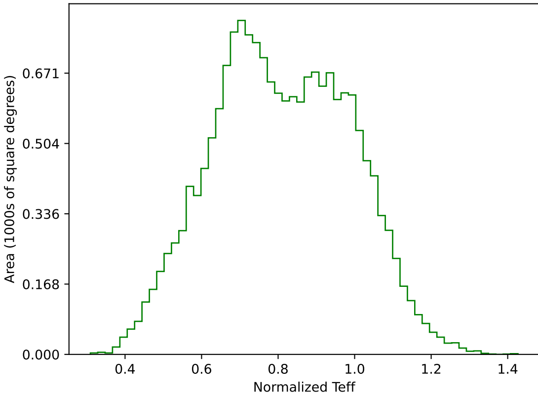
extra_ss_neo4_v3.4_10yrs WFD g band: Normalized Teff
