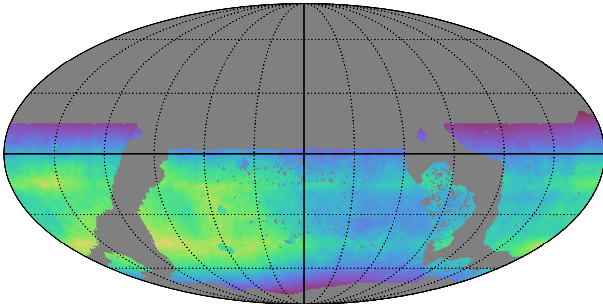
extra_ss_neo4_v3.4_10yrs WFD all bands: Normalized Teff
