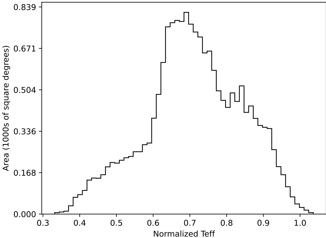
extra_ss_neo4_v3.4_10yrs WFD all bands: Normalized Teff
