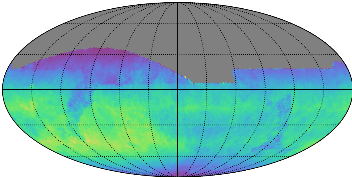
extra_ss_neo4_v3.4_10yrs All sky z band: Normalized Teff
