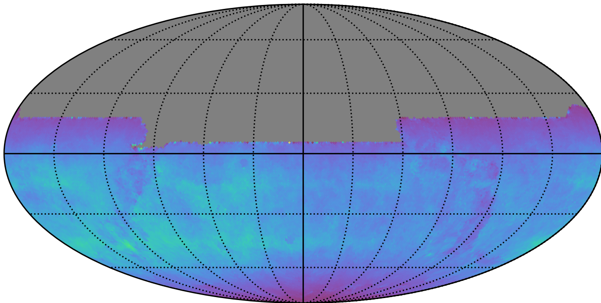
extra_ss_neo4_v3.4_10yrs All sky y band: Normalized Teff
