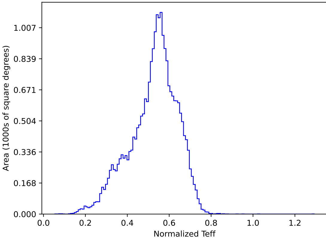
extra_ss_neo4_v3.4_10yrs All sky y band: Normalized Teff
