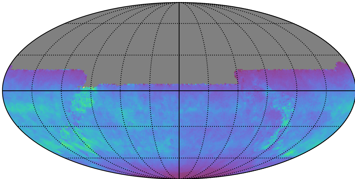
extra_ss_neo4_v3.4_10yrs All sky u band: Normalized Teff
