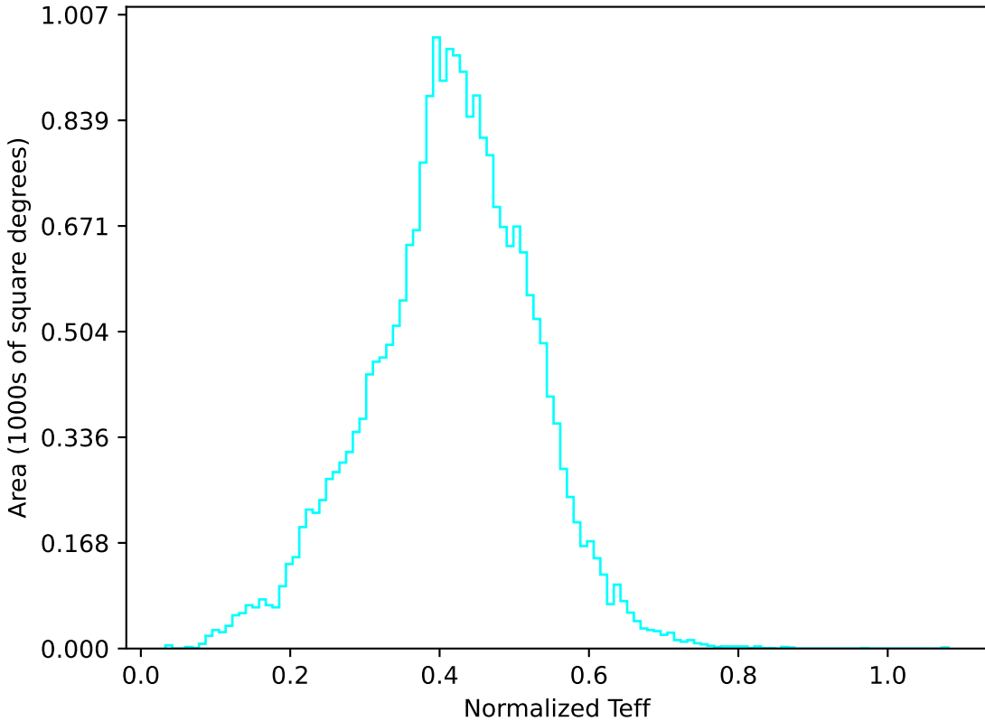
extra_ss_neo4_v3.4_10yrs All sky u band: Normalized Teff
