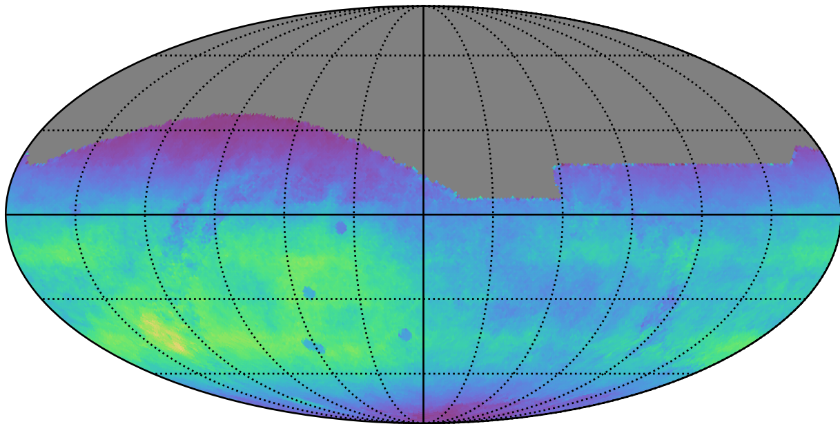
extra_ss_neo4_v3.4_10yrs All sky r band: Normalized Teff
