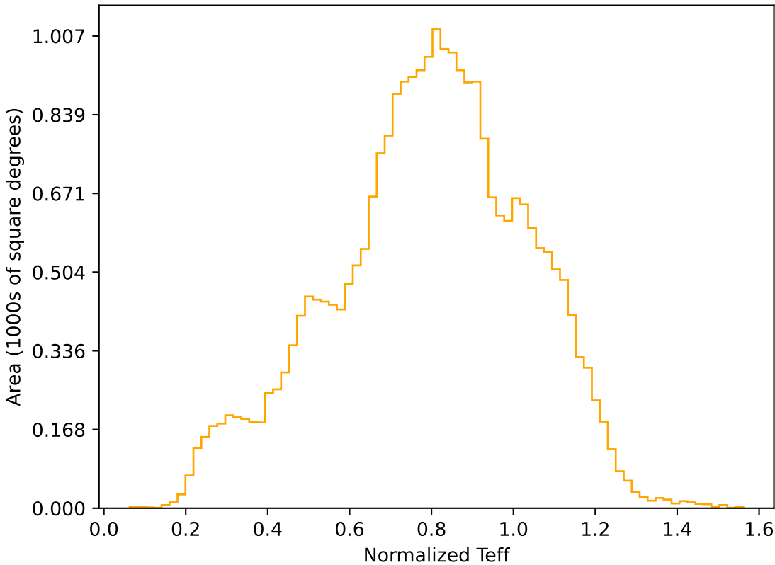
extra_ss_neo4_v3.4_10yrs All sky r band: Normalized Teff
