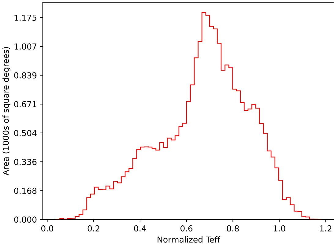
extra_ss_neo4_v3.4_10yrs All sky i band: Normalized Teff
