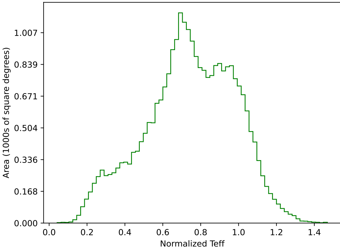
extra_ss_neo4_v3.4_10yrs All sky g band: Normalized Teff
