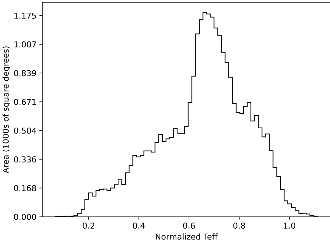
extra_ss_neo4_v3.4_10yrs All sky all bands: Normalized Teff
