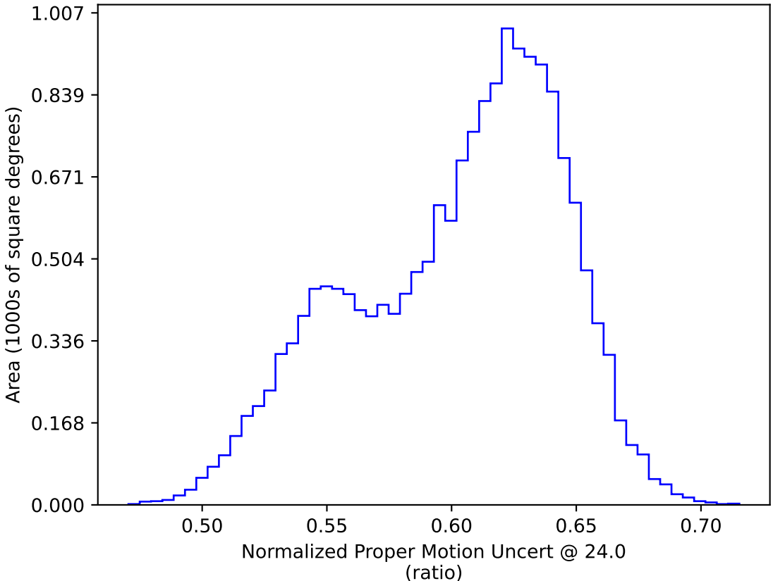
extra_ss_neo4_v3.4_10yrs WFD: Normalized Proper Motion Uncert @ 24.0
