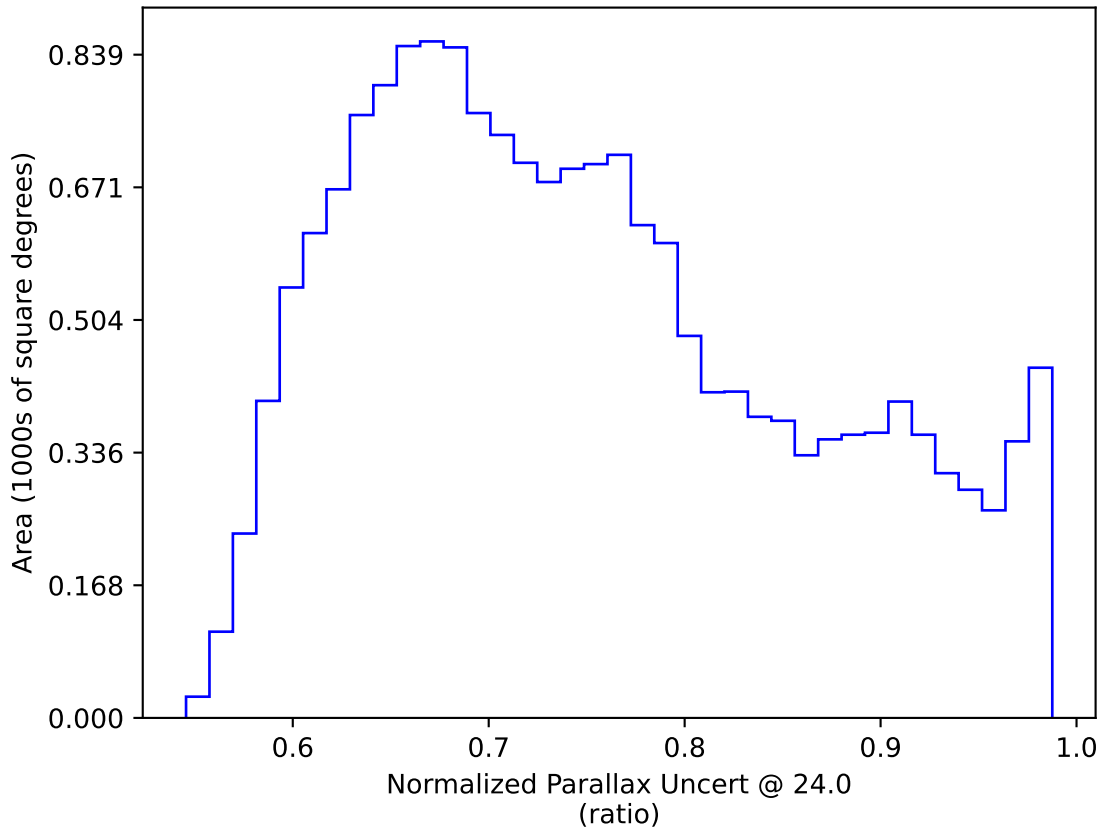
extra_ss_neo4_v3.4_10yrs WFD: Normalized Parallax Uncert @ 24.0
