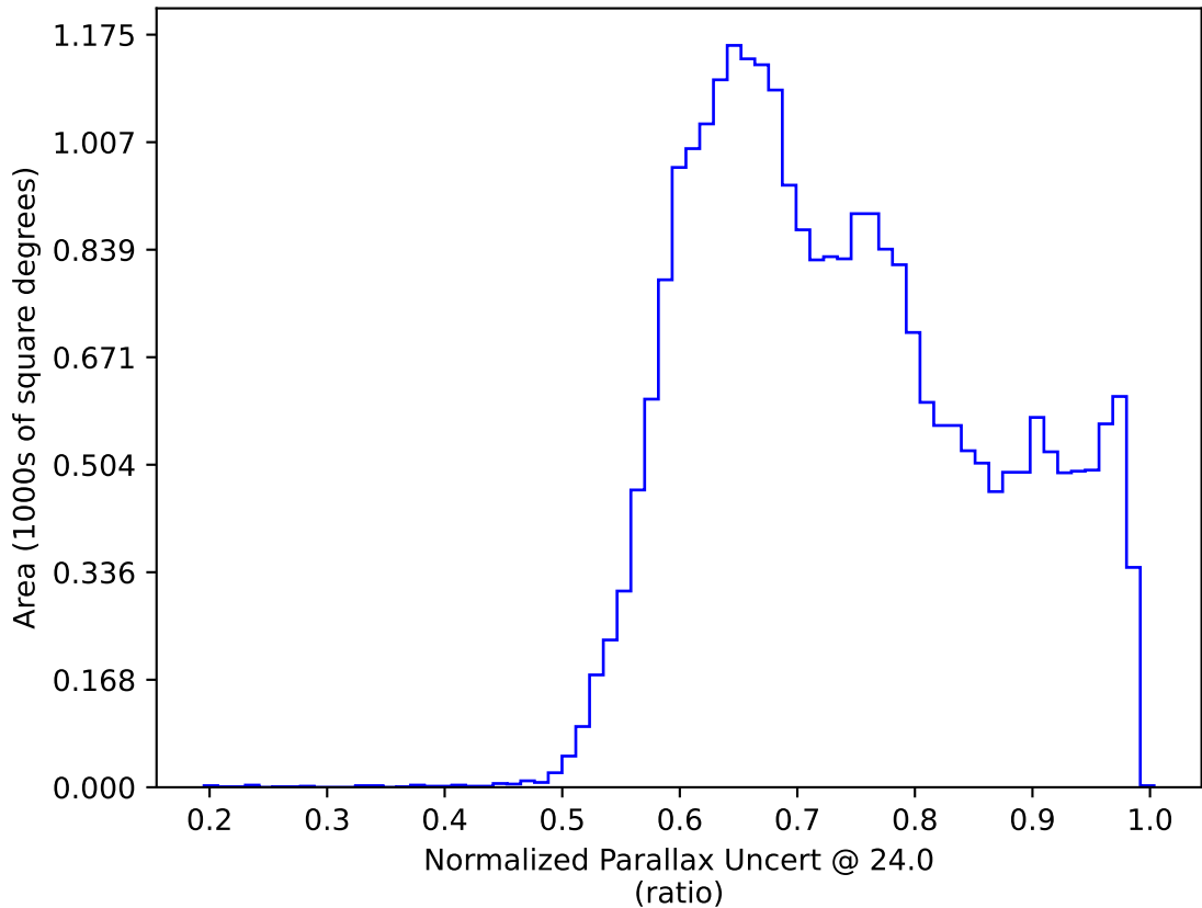
extra_ss_neo4_v3.4_10yrs All sky: Normalized Parallax Uncert @ 24.0
