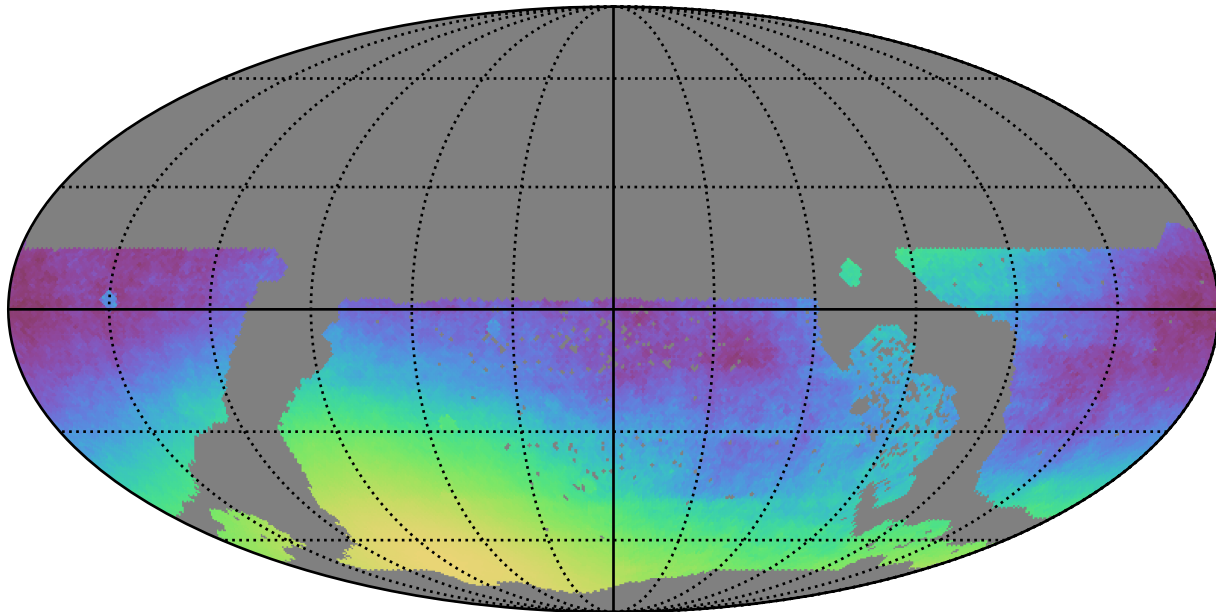
extra_ss_neo4_v3.4_10yrs WFD: Normalized Parallax Uncert @ 22.4
