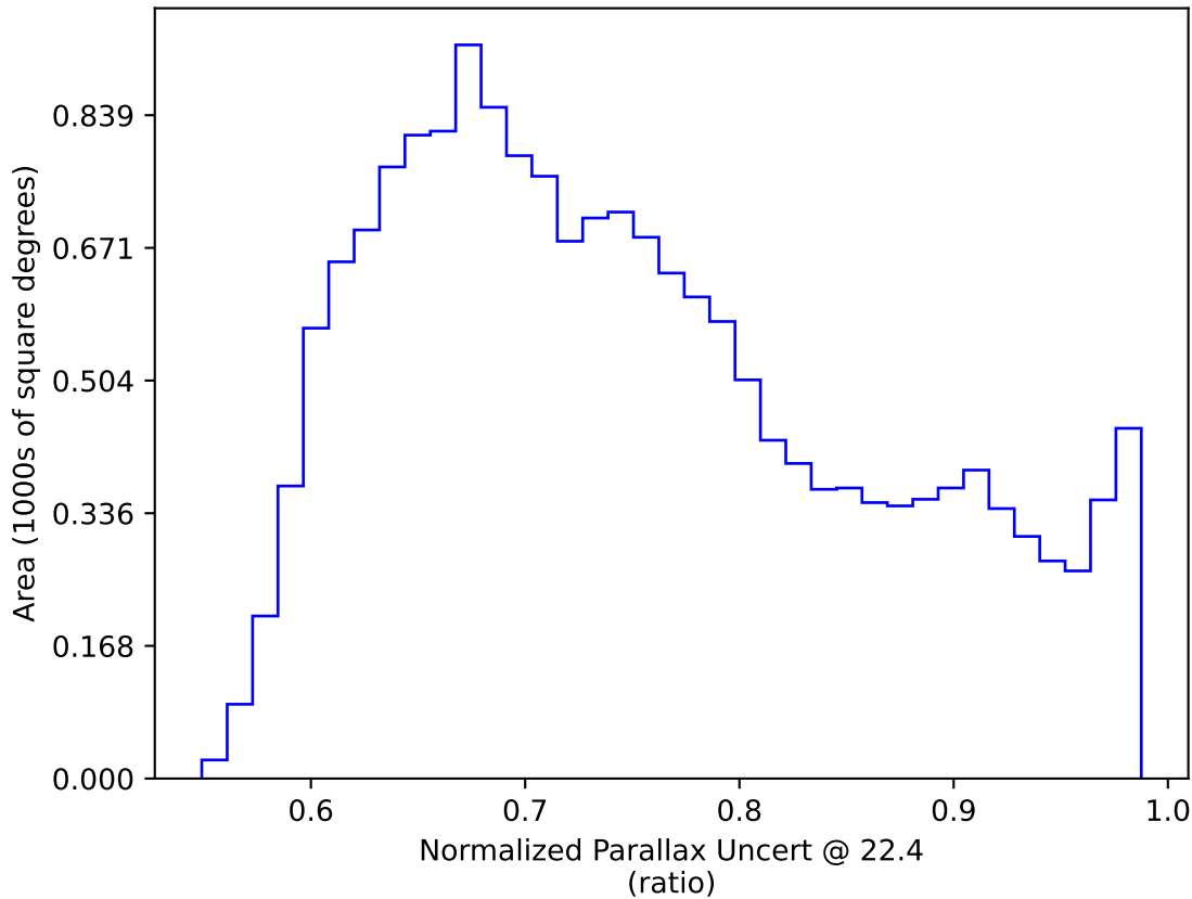
extra_ss_neo4_v3.4_10yrs WFD: Normalized Parallax Uncert @ 22.4
