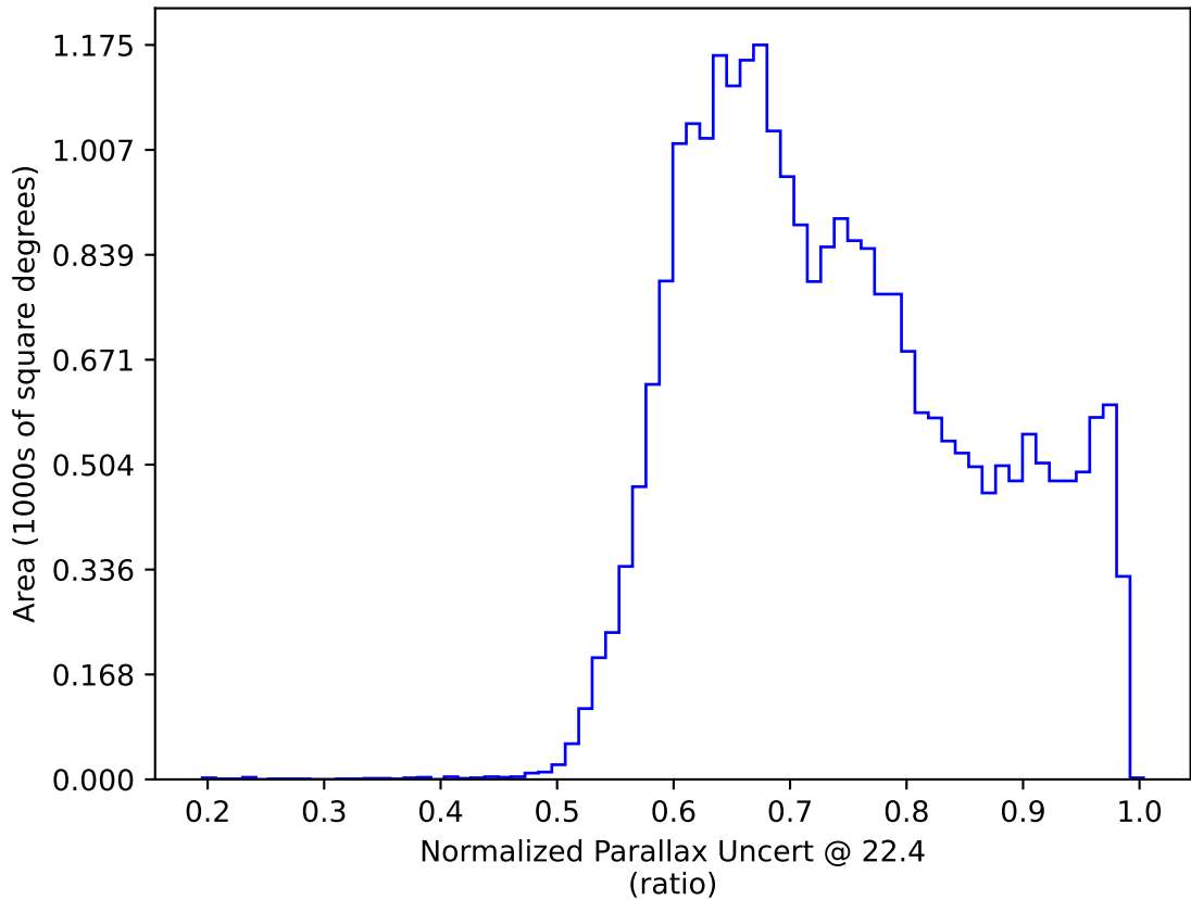
extra_ss_neo4_v3.4_10yrs All sky: Normalized Parallax Uncert @ 22.4
