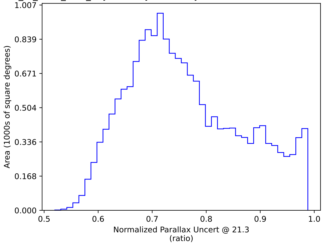
extra_ss_neo4_v3.4_10yrs WFD y band only: Normalized Parallax Uncert @ 21.3
