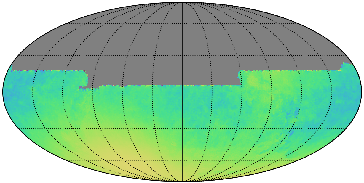
extra_ss_neo4_v3.4_10yrs All sky y band only: Normalized Parallax Uncert @ 21.3
