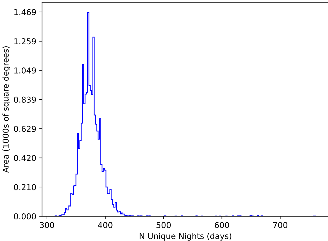
extra_ss_neo4_v3.4_10yrs WFD all bands: N Unique Nights
