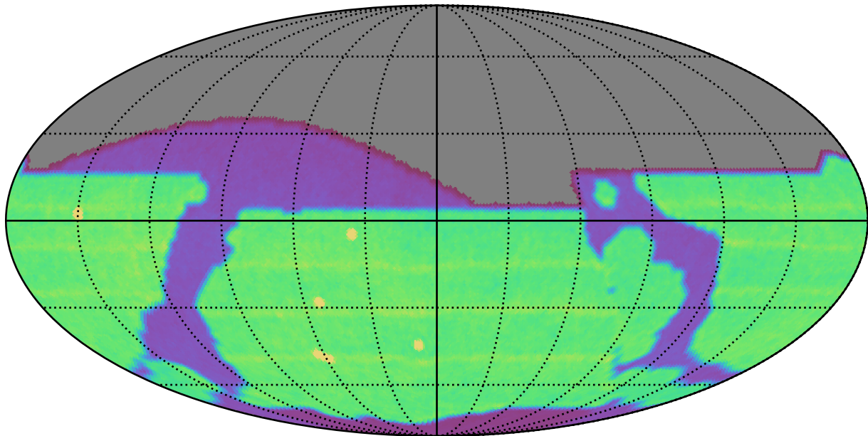
extra_ss_neo4_v3.4_10yrs All sky all bands: N Unique Nights
