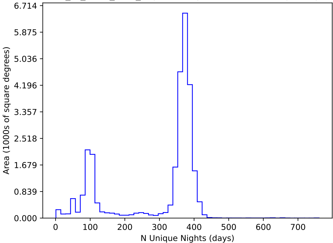
extra_ss_neo4_v3.4_10yrs All sky all bands: N Unique Nights
