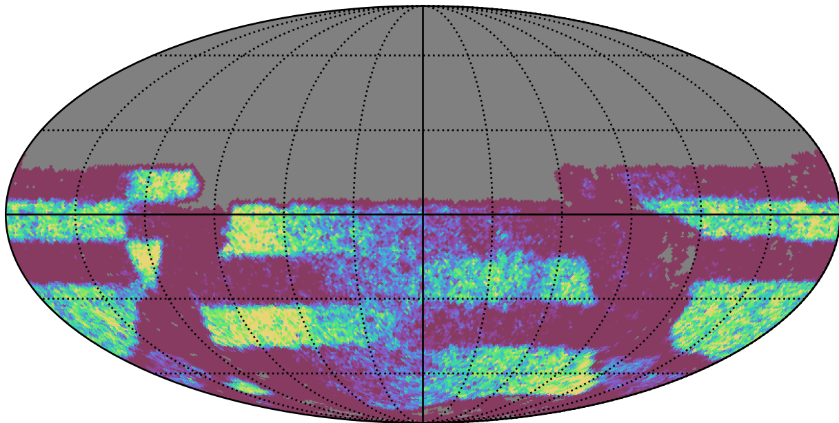
extra_ss_neo4_v3.4_10yrs Yr 3-4 y band: NVisits
