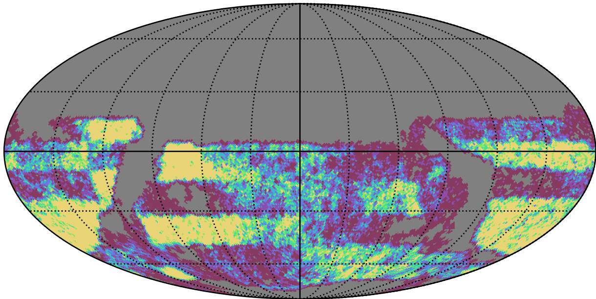
extra_ss_neo4_v3.4_10yrs Yr 3-4 u band: NVisits
