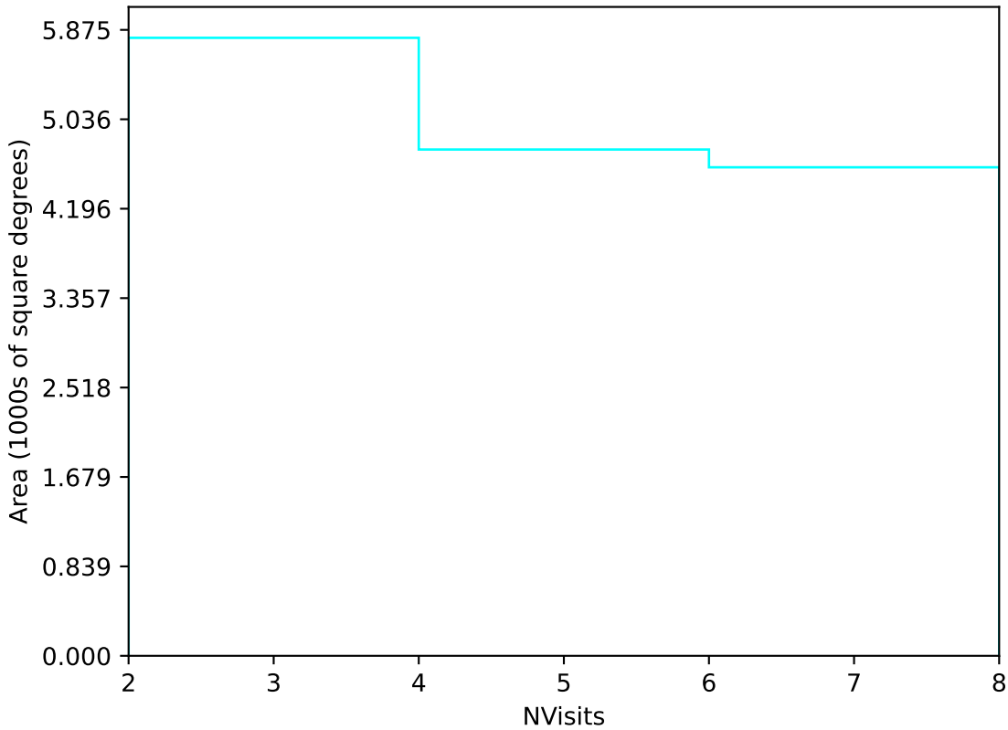
extra_ss_neo4_v3.4_10yrs Yr 3-4 u band: NVisits
