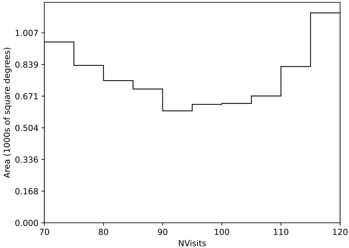
extra_ss_neo4_v3.4_10yrs Yr 3-4 all bands: NVisits
